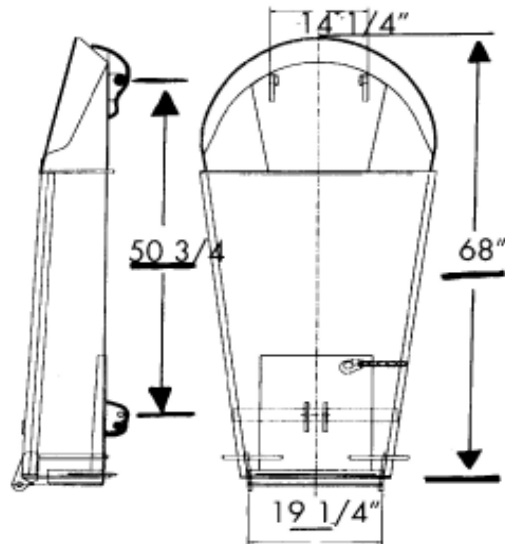
C 4000 New Style Smith Main Chute
