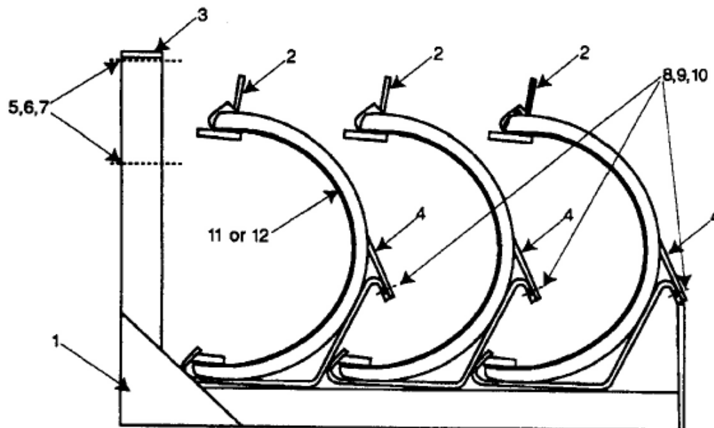
C 1002 ASSY Chute Hold Down Assy
