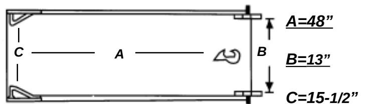
C 2000 Old Style Smith Extension Chute
