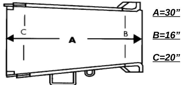
C 3007 New Style Smith Foldover Chute
