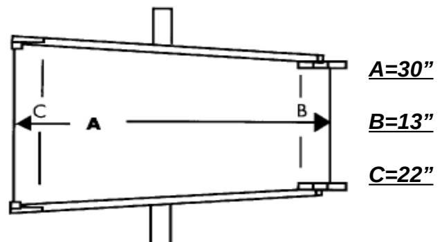
C 3006 Old Style Smith Foldover Chute
