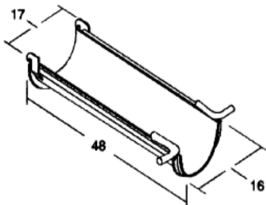
C2011 Current MTM Production Extension Chute 4 foot steel
