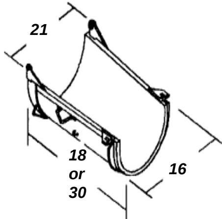
C3009 Current MTM Production Foldover 96
