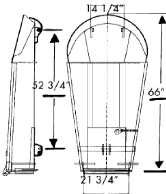
C 4001 Old Style Smith Main Chute
